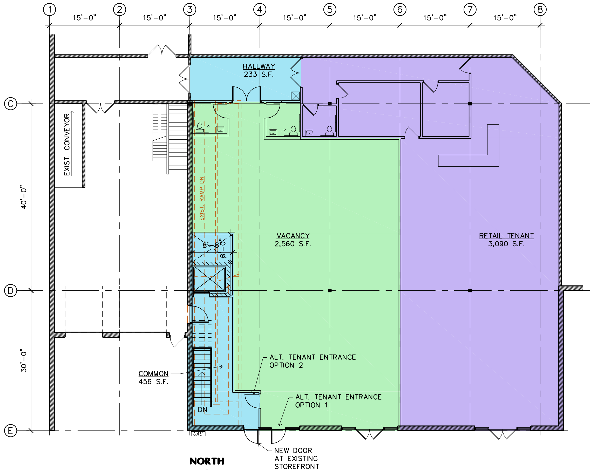
1 MAIN FLOOR PLAN A1 SCALE: 3/32" = 1'-0"
